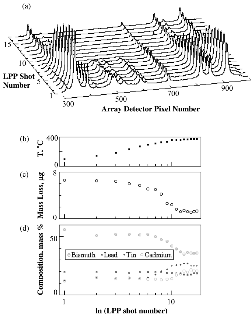
Fig. 4. Results from the seventeen consecutive LPP plume runs, as shown in Fig. 2, are presented as a function of the shot number: (a) emission spectra from the top surface of the Wood's alloy specimen, as it is reheated up to 374°C; (b) actual specimen temperature; (c) mass loss per LPP shot; and (d) elemental composition of each LPP plume. The shot number axis is represented logarithmically. The wavelength axis for (a) is organized in the same manner as described in the caption of Fig. 2.
