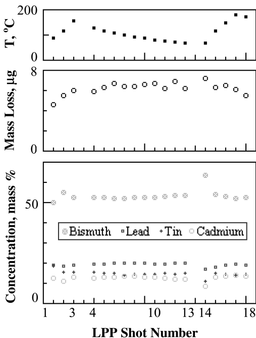
Fig. 3. Measured elemental concentration and mass loss for the thermally cycled Wood's alloy specimen of Fig. 2. The results are derived from the set of spectra shown in Fig. 2. The following emission lines are used: 4057.807 Å PbI (pixel #348) for lead; 4524.74 Å SnI (pixel #702) for tin; 4722.52 Å BiI (pixel #858) for bismuth; and 4678.149 Å CdI (pixel #823), and 4799.912 Å CdI (pixel #920) for cadmium.
