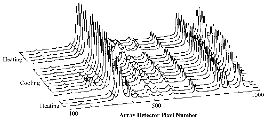
Fig. 2. LPP plume emission spectra from the top surface of a Wood's alloy specimen, which has been heated to melting, followed by cooling, heating and cooling, according to a protocol described in the text. The actual specimen temperature is shown in Fig. 3. The array detector pixel addresses are shown along the wavelength axis. The wavelength increases linearly with increasing pixel address, where pixel #348 and #920 correspond to 4057.807 and 4799.912 Å, respectively.
