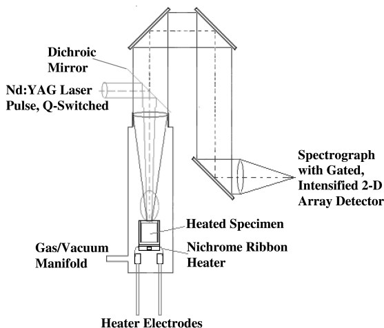
Fig. 1. Schematic diagram of the specimen vacuum chamber, which is vertically positioned. At the top is the shared optics for laser beam delivery to the specimen and for collection and transfer of LPP plume emissions for quantitative spectroscopy. A high energy density dichroic mirror is used for this purpose. A spectrograph and gated intensified 2-D array detector facilitates time- and space-resolved measurement of the LPP plume spectrum. The specimen is contained in a crucible inside the chamber, which is supported and heated by a Nichrome ribbon heater. The chamber is filled with argon to 150 Torr during the LPP analysis runs in order to suppress darkening of the optical surfaces due to alloy vapor condensation.
