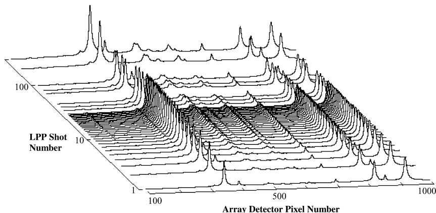
Fig. 5. Selected LPP emission spectra from a 300-shot sequence of LPP analysis carried out for a Wood's alloy specimen in a solid form near room temperature. The specimen had been processed through three rounds of heating and cooling. The detailed history of thermal cycling is given in the text. The highest specimen temperature was 371°C. The wavelength axis is organized in the same manner as described in the caption of Fig. 2.
